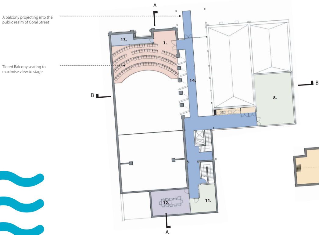
Concept: - Level 1
